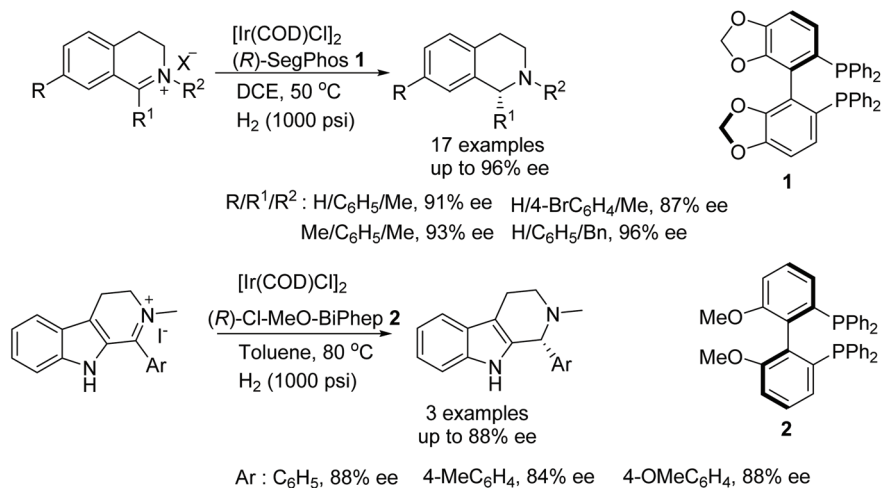
Fig. 1 AH of N -alkyl tetrahydroisoquinolines and N -alkyl tetrahydro-β-carbolines.
