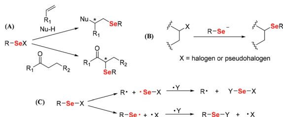
Scheme 1 The reactivity of electrophilic, nucleophilic and radical reactions of organoselenium compounds. 28,29 (A) Electrophilic reactions; (B) nucleophilic reactions; and (C) radical reactions.
