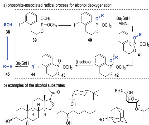
Fig. 8 Phosphite-associated deoxygenation of alcohols.
