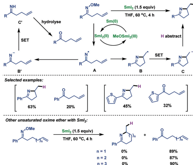
Scheme 31 Zhang's \text{Sml}_2 promoted hydroimination of \gamma,\delta -unsaturated oxime ethers.
