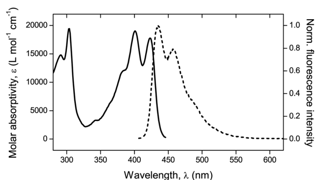
Fig. 3 UV-vis absorption spectrum (solid line) and normalized fluorescence emission spectrum (dashed line). \lambda_{exc} = 372 nm.
