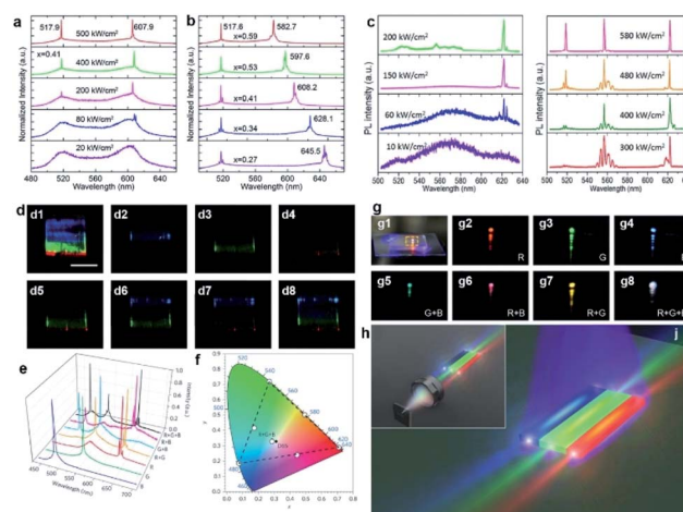
Fig. 9 Monolithic multi-color lasers based on single lateral hetero-nanobelts. (a) Power-dependent PL spectra of a CdS–CdS Se tri-lane hetero-nanobelt. (b) Lasing spectra from CdS–CdS Se tri-lane hetero-nanobelts with different S/Se ratios ( x ) in the middle lanes. (c) Power dependent PL spectra of a CdS–CdS Se lateral graded nanobelt. (d) Real-color images of a single ZnCdS Se multi-lane nanobelt, under low pumping (d1) and above-threshold pumping (d2–d8). (e) Corresponding PL spectra acquired from panels d2 to d8. (f) Chromaticity of the lasing peaks extracted from the spectra in (e). (g1) Photograph of the mixed emission colour. (g2–g8) Photographs of the enlarged dashed-box region in (g1) when the different combinations of segments are pumped as indicated by the labels inside each figure, creating the mixed far-field emission colours red, green, blue, yellow, cyan, magenta and white. The top dots in each photograph are the direct images of laser emission, while the tails under these dots are the reflections from the substrate. (h) Schematic diagram for achieving a monolithic white laser from an individual multi-lane hetero-nanobelt. (a and b) Reproduced with permission. 45 Copyright 2012, American Chemical Society. (c) Reproduced with permission. 49 Copyright 2016, Springer. (d–h) Reproduced with permission. 15 Copyright 2015, Nature Publishing Group.
