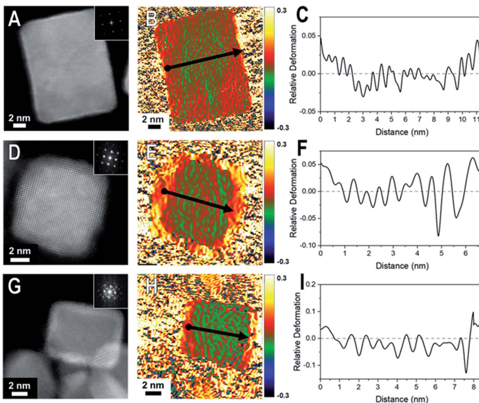
Fig. 2 HAADF-STEM images and corresponding GPA for the thin (2–4 ML) shelled samples (A–C) Pd@Pt, (D–F) Rh@Pd, and (G–I) Rh@Pt nanocubes. The first column consists of the HAADF-STEM images of the nanocrystal examined by GPA. The second column contains the corresponding GPA colors maps which correspond to the in-plane strain ( \epsilon_{xx} ) field (which is the strain in the plane of the crystal face) where the intensity scale shows relative deformation. The third column contains line profiles of the lattice difference determined by GPA with the line profile locations indicated by arrow in the GPA color maps where the start of the line profile begins at the dot and ends at the arrow head.
