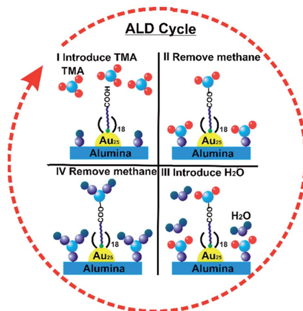
Fig. 11 General scheme of alumina deposition over Au 25 (MUA) 18 /Al 2 O 3 by atomic layer deposition. Reprinted with permission from ref. 111. Copyright 2018 American Chemical Society.
