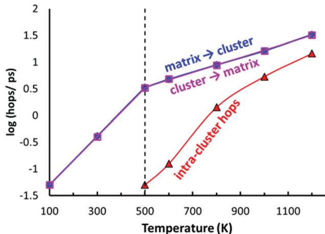
Fig. 10 Temperature dependences of the site-specific hop frequencies in AIMD simulations of \text{Na}_{11}\text{Sn}_2\text{PS}_{12} . Hops are classified into hops from the (\text{Na}_2)_4(\text{Na}_3)_2\text{Na}_6 site cluster to the interconnecting “matrix sites” Na1, Na4 or Na5 (magenta open squares), vice versa (blue filled diamonds), or intra-cluster rearrangements within the vacancy-rich (\text{Na}_2)_4(\text{Na}_3)_2\text{Na}_6 cluster (red triangles). The broken vertical line marks the onset of \text{PS}_4 rotational disorder above 500 K.
