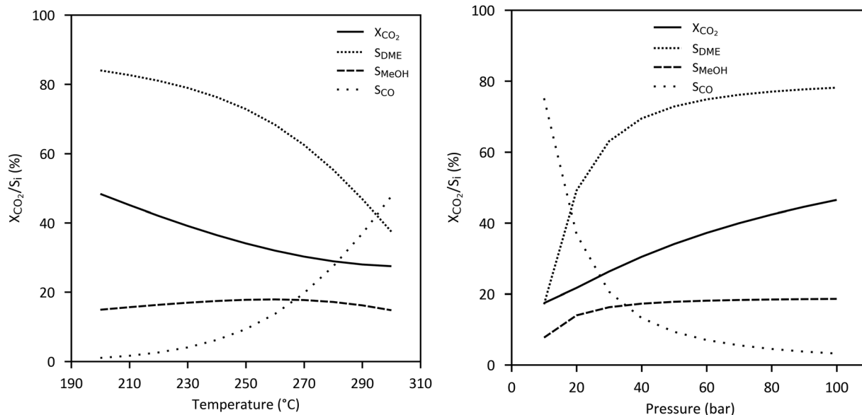
Fig. 13 Equilibrium conversion of CO 2 ( = [CO_{2,in} - CO_{2,out}]/CO_{2,in} ) and selectivity of DME, methanol and CO ( S_i = i/[CO_{2,in} - CO_{2,out}] , with i = 2 \times DME/MeOH/CO , based on amount of C-atoms) dependent on (a) temperature and (b) pressure ( H_2 : CO_2 = 3 : 1 , based on Aspen Plus Simulation).
