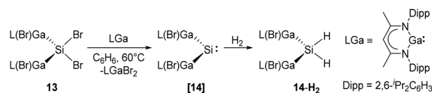
Scheme 9 Synthesis of 14-H 2 by the acyclic silylene 14 .
