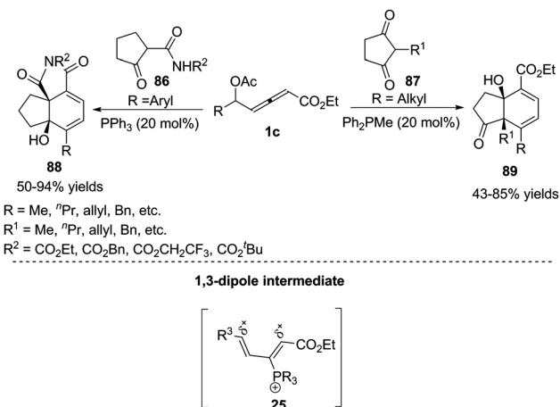
Scheme 28 Phosphine-catalysed (4+2) annulations of \delta -acetoxy allenones and ketones.
