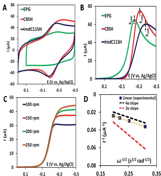
Fig. 3 (A) CV data of Fe ^{III}Cl -MARG over the EPG electrode (green), C_8SH SAM- (red) and Imd C_{11}SH SAM (blue) modified Au electrodes in the absence of O _2 in pH 7 phosphate buffer with KPF _6 supporting electrolyte at a scan rate of 1 V s ^{-1} ; (B) LSV data of the complex in air saturated pH 7 phosphate buffer over EPG (green), C_8SH SAM (red) and Imd C_{11}SH SAM (blue) at 0 rpm at a scan rate of 50 mV s ^{-1} ; (C) RDE plots of the catalyst over the EPG electrode for multiple rotations at a scan rate of 50 mV s ^{-1} ; (D) K–L plot of the catalyst at a potential of –0.5 V.
