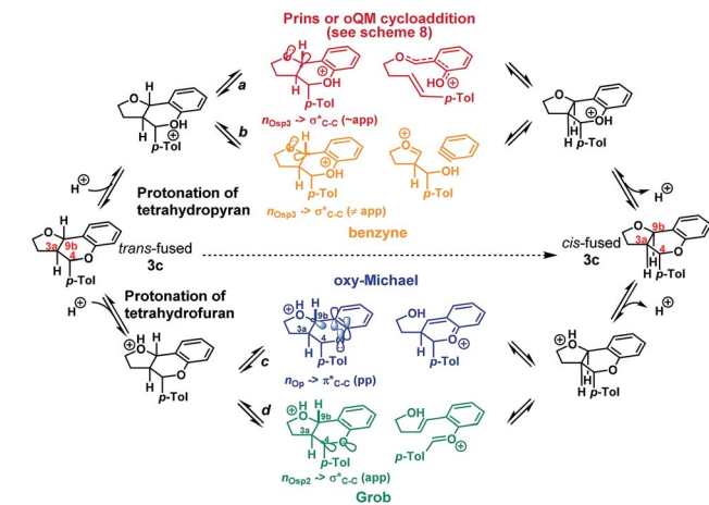
Scheme 4 Potential pathways for isomerization.
