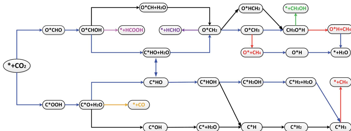
Scheme 1 Most likely reaction pathways for the electroreduction of CO 2 on TM-B 12 .
