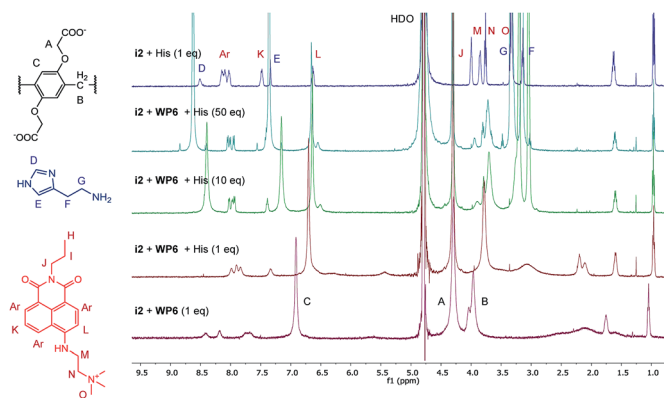
Fig. 8 ^1H -NMR spectra (500 MHz, D_2O , 0.5 mM) of the indicator displacement of i2 - WP6 mixture in the presence of histamine in different concentrations. The uppermost spectrum is a mixture of i2 and histamine.
