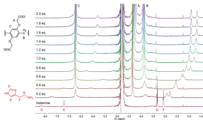
Fig. 7 ^1H -NMR spectra (500 MHz, D_2O , 0.5 mM) of histamine in the presence of 0 to 2.0 equivalents of WP6 .
