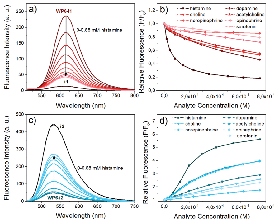
Fig. 6 Indicator displacement of the complexes with various neurotransmitter analytes in HEPES buffer (pH 7.4). (a) Fluorescence spectra of WP6 \cdot i1 ( 0.9 \mu M i1 , 5.8 \mu M WP6 , \lambda_{ex} : 482 nm) upon addition of histamine (0 to 0.68 mM) (b) relative fluorescence values of WP6 \cdot i1 at 615 nm upon addition of different analytes (c) fluorescence spectra of WP6 \cdot i2 ( 0.9 \mu M i1 , 126 \mu M WP6 , \lambda_{ex} : 438 nm) upon addition of histamine (0 to 0.68 mM) (d) relative fluorescence values of WP6 \cdot i2 at 533 nm upon addition of different analytes.
