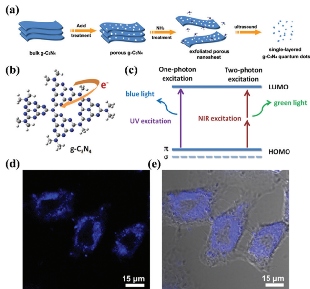
Fig. 3 Biological imaging based on g-CN 4 luminescence. (a) g-CN 4 are formed into QDs that have three-dimensional nanostructures using physical and chemical methods, such as acid–base treatment and ultrasound. (b) In g-CN 4 in the graphitic phase, the tri-triazine structure produces free electrons on their surface. (c) Fluorescence can be achieved using different excitation frequencies that excite blue and green light with single photons and multiple photons, respectively. (d) g-CN 4 under a conjugated focus microscope emit blue light. Reproduced with permission. 12 Copyright 2014, Wiley Online Library.
