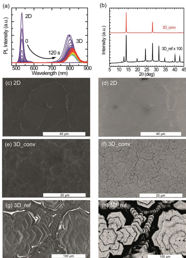
Fig. 3 2D–3D conversion kinetics and structural and morphological characterization of the converted and reference 3D perovskite films, all fabricated by the doctor-blade coating technique. (a) In situ photoluminescence (PL) emission spectra showing the conversion kinetics of the evolution from 2D to 3D perovskites, (b) X-ray diffraction patterns of the converted and the reference film fabricated by doctor-blade coating. (c–h) Four SEM images showing the surface topography and compositional properties of the 2D \text{PEA}_2\text{PbI}_4 , the converted and the reference 3D \text{FAPbI}_3 perovskite films. (c, e and g) Secondary electron and (d, f and h) backscattered electron images of the 2D, converted and reference 3D perovskite films, respectively.
