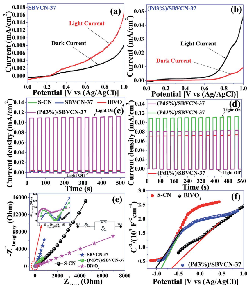
Fig. 7 LSV curves of (a) SBVCN-37 and (b) (Pd3%)/SBVCN-37 in the dark and under light illumination. (c and d) Transient photocurrent ( i – t ) of all the photocatalysts, (e) EIS profiles (inset shows enlarged profiles at the low frequency region and simulated equivalent circuit), and (f) Mott–Schottky plots of BiVO 4 , S-CN, and (Pd3%)/SBVCN-37 at the constant frequency of 1000 Hz.
