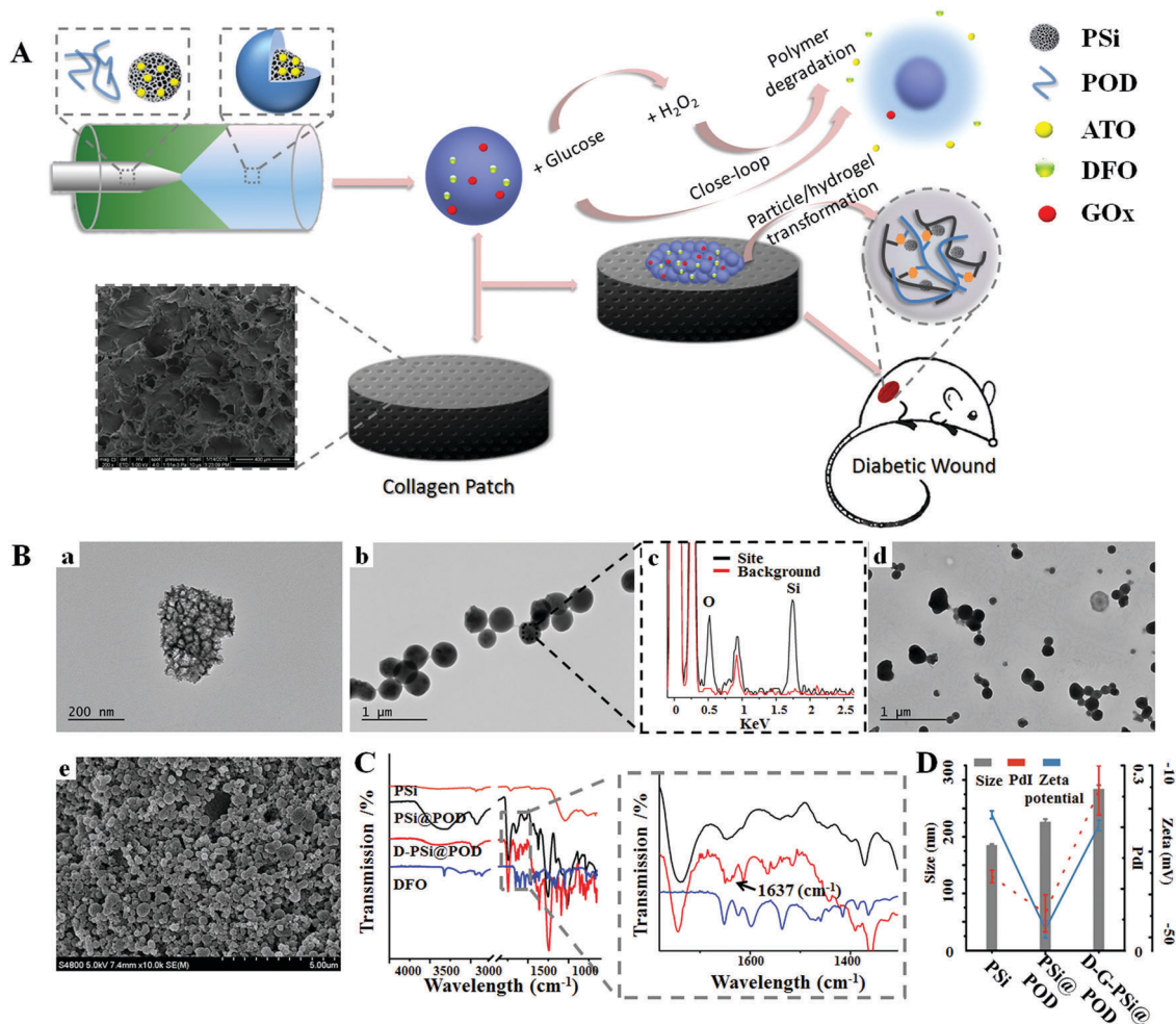
Fig. 1 Preparation and characterization of DFO, GOx conjugated, ATO loaded nano-hybrid (D-G-PSi@POD). (A) Schematic illustration of the construction of glucose responsive delivery system and the orchestrated cascade for diabetic wound care. The detrimental side product of H 2 O 2 , was utilized and consumed, further aiding the close-loop system. (B) TEM/SEM images showing morphologies of (a) PSi, (b) PSi@POD and (c) their respective EDX spectra at particle site and the background, (d) D-G-PSi@POD and (e) D-G-PSi@POD embedded on the collagen patch without obvious morphology changes. (C) FTIR spectra of PSi, PSi@POD, D-PSi@POD and DFO, suggesting a successful encapsulation and Schiff-base formation. (D) Size, PDI and zeta-potential shift during each step of synthesis, suggesting a successful modification in each step.
