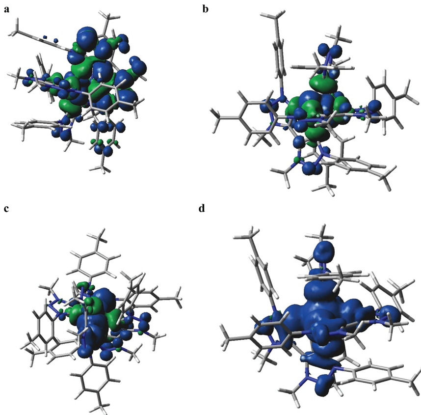
Fig. 6 Spin density plots (isovalued 0.0004) of selected Fe II (btz) 3 and Fe III (btz) 3 states from B3LYP*/6-311G(d)|MeCN calculations. Specific oxidation and electronic state assignments: (a) Fe II : 3 MLCT, (b) Fe III : 2 GS, (c) Fe III : 4 MC, (d) Fe III : 6 MC.
