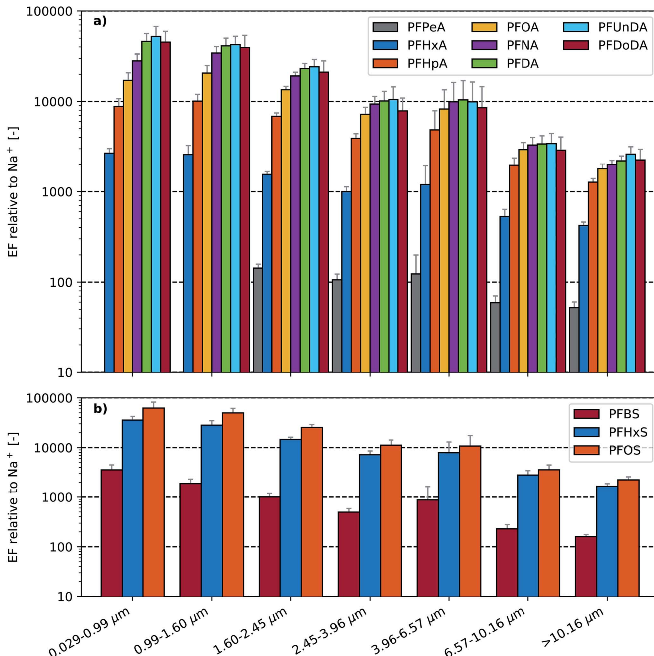
Fig. 2 Enrichment factor, EF(X), relative to \text{Na}^+ of (a) perfluoroalkyl carboxylic acids (PFCAs) and (b) perfluoroalkane sulfonic acids (PFSA) as a function of particle aerodynamic diameter (experiment A). Note that PFPeA was not detectable in the two lowest stages of the impactor so no EF could be calculated. Here error bars represent 1 standard deviation following propagation of the standard deviation of the \text{Na}^+ and PFAA concentrations measured in the seawater and aerosol samples.
