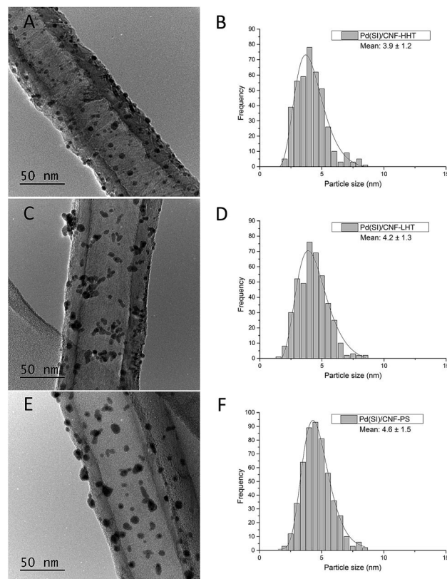
Fig. 7 Bright field TEM micrographs and corresponding histograms of the particle size distributions for the fresh catalysts prepared by sol-immobilisation. (A and B) \text{Pd}_{\text{Si}}/\text{CNF-HHT} , (C and D) \text{Pd}_{\text{Si}}/\text{CNF-LHT} , and (E and F) \text{Pd}_{\text{Si}}/\text{CNF-PS} .
