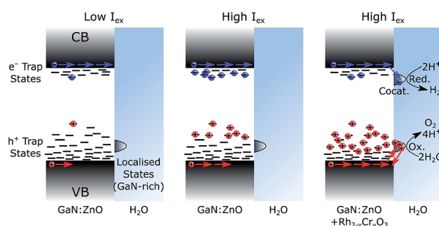
Fig. 7 Schematic representation of trap state filling. The left case shows \text{GaN:ZnO} photoexcited with low light flux, the middle case shows \text{GaN:ZnO} photoexcited with high light flux, and the right case shows \text{GaN:ZnO/Rh}_{2-y}\text{Cr}_y\text{O}_3 photoexcited with high light flux. Charge distribution reflects a thermalized population, as expected under continuous solar irradiation.
