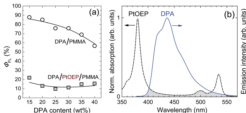
Fig. 1 (a) Fluorescence quantum yield of DPA as a function of its concentration in the PMMA matrix without (circles) and with (squares) PtOEP ( c_{PtOEP} = 0.05\text{ wt\%} ). The excitation wavelength ( \lambda_{ex} = 405\text{ nm} ) corresponds to the absorption maximum of DPA. Lines are guides to the eye. (b) Normalized absorption (dashed line) and emission spectra (solid line) of melt-processed PtOEP/PMMA ( c_{PtOEP} = 0.05\text{ wt\%} ) and DPA/PMMA ( c_{DPA} = 25\text{ wt\%} ) films, respectively. The shaded area indicates spectral overlap.
