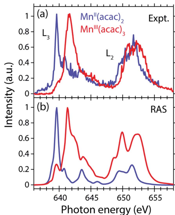
Fig. 3 Comparison of (a) measured and (b) calculated partial-fluorescence-yield (PFY) Mn L-edge absorption spectra of Mn II (acac) 2 and Mn III (acac) 3 . (a) Experimental spectra of ~0.05 mol l -1 Mn II (acac) 2 solution in ethanol and ~0.1 mol l -1 Mn III (acac) 3 solution in acetylacetone. (b) Calculated spectra from the restricted active space (RAS) calculations with photon energies of the Mn II (acac) 2 spectrum shifted to match the experimental spectrum at the L 3 -edge maxima, while keeping the relative photon energies of Mn II (acac) 2 and Mn III (acac) 3 spectra as calculated. In all spectra the intensities were normalized to one at maximum.
