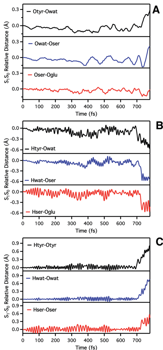
Fig. 3 Time evolution of S_1-S_0 relative distances (Å) involved in the ESPT. (A) Oxygen-oxygen distances: Otyr-Owat (top), Owat-Oser205 (middle) and Oser-Oglu (bottom); (B) hydrogen-acceptor oxygen distances: Htyr-Owat (top), Hwat-Oser205 (middle) and Hser-Oglu222 (bottom); (C) hydrogen-donor oxygen distances: Otyr-Htyr (top), Owat-Hwat (middle) and Oser205-Hser205 (bottom).
