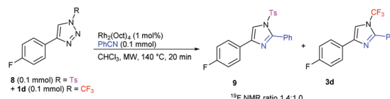
Scheme 5 Transannulation competition experiment revealing comparative reactivity of N -trifluoromethyl and N -tosyl triazoles with benzocyanide.
