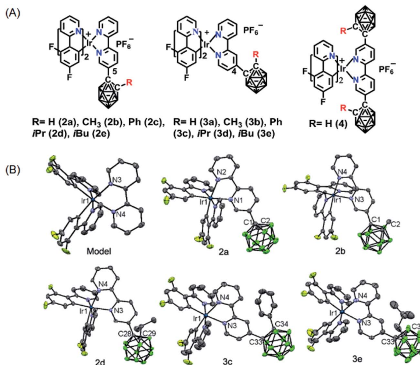
Fig. 1 (A) Nomenclatures of carborane-modified iridium(III) complexes; (B) ORTEP diagrams of complexes Model, 2a, 2b, 2d, 3c, and 3e. H atoms, solvent molecules, and \text{PF}_6^- anions are omitted for clarity.
