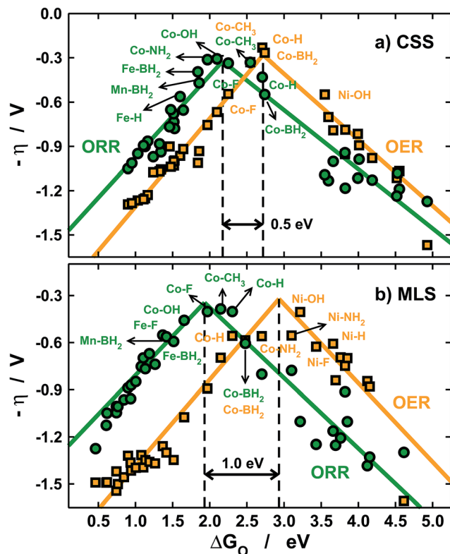
Fig. 6 Volcano-type activity plots for the ORR (green) and the OER (orange). The overpotential ( \eta ) is plotted against the adsorption energies of ^*O , see Section S2 in the ESI† (a) Using a constant-shift solvation correction (CSS) from ref. 11 and 26 and (b) using the metal- and ligand-dependent solvation corrections (MLS) calculated in this study. The black dashed lines mark the top of the OER and ORR volcanoes and show that different solvation treatments lead to different activity predictions.
