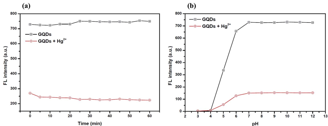
Fig. 5 (a) The changes in the fluorescence intensity of the GQDs at different reaction times. Conditions: 4 μM Hg 2+ in 0.1 M phosphate buffer at a pH of 7.0 and (b) the changes in the fluorescence intensity of the GQDs at different values of pH. Conditions: 4 μM Hg 2+ and 5 min reaction time.
