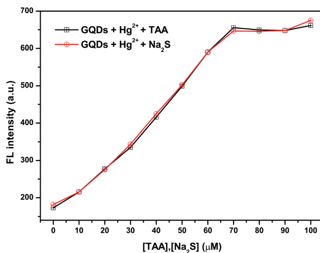
Fig. 6 The effect of different concentrations of TAA or Na 2 S on the fluorescence intensity of the Hg 2+ –GQDs.
