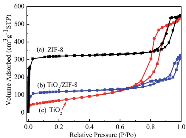
Fig. 4 N 2 adsorption–desorption isotherms of (a) ZIF-8, (b) TiO 2 /ZIF-8, (c) TiO 2 beads.
