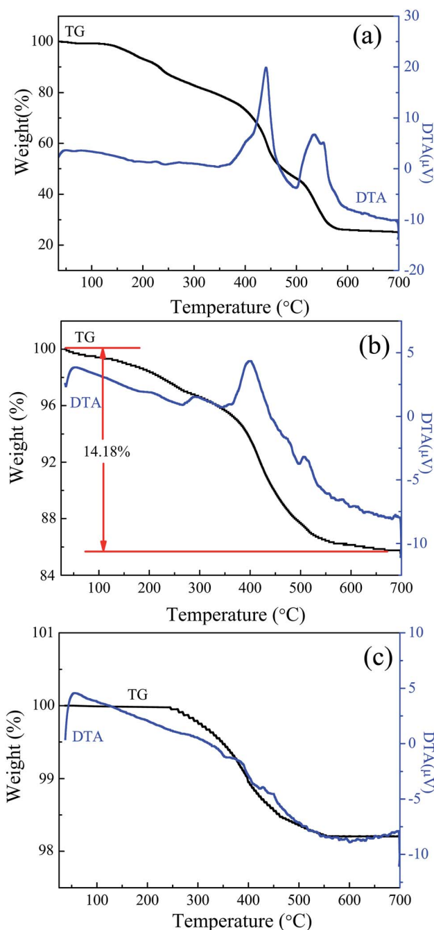
Fig. 5 TG (black curve) and DTA (blue curve) analysis of (a) ZIF-8, (b) TiO 2 /ZIF-8, (c) TiO 2 beads.
