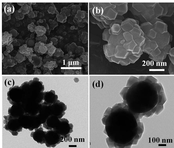
Fig. 3 (a) and (b) FE-SEM images, and (c) and (d) TEM images of the TiO 2 /ZIF-8 hybrid beads.
