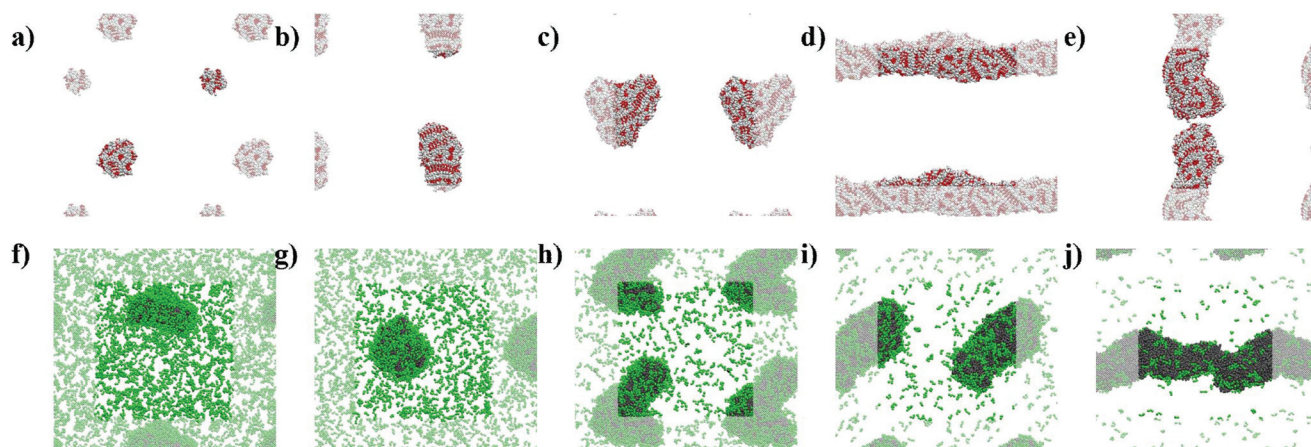
Fig. 3 Simulation snapshots at 10 \mu s for: (a) F_6^{100} , (b) F_6^{200} , (c) F_6^{300} , (d) F_6^{400} , (e) F_6^{500} , (f) F-L^{100-1500} , (g) F-L^{200-1200} , (h) F-L^{300-900} , (i) F-L^{400-600} and (j) F-L^{500-300} . (a–e) F_6 systems show backbone beads in red and side chain beads in white; (f–j) and F-L systems show F_6 molecules in grey and L_2 in green. Periodic images are transparent for all the systems.
