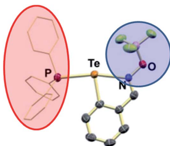
Fig. 13 N–Te...P chalcogen bond. Strong chalcogen bonding capability of Te is activated by coordination of \text{N} -oxide, and further enhanced by Lewis acid coordination of the \text{BF}_3 group to the oxygen (blue circle). Phosphine ( \text{PPh}_3 , red ellipse) serves as the (Lewis basic) chalcogen bond acceptor. Adapted from DOI: 10.1039/c7fd00075h with permission from The Royal Society of Chemistry.
