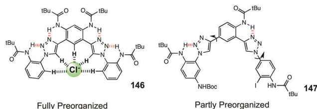
Fig. 40 The arytriazole foldamer 16 is fully pre-organized by four contiguous hydrogen bonds on its periphery. Receptor 16 favours a conformation that is optimal for anion binding, and subsequent transmembrane anion transport, by the use of \text{CH}\cdots\text{anion} hydrogen-bonds. The control compound 17 , because it lacks the same degree of pre-organization as 16 , is conformationally more flexible and does not bind or transport chloride anion as well as foldamer 16 .
