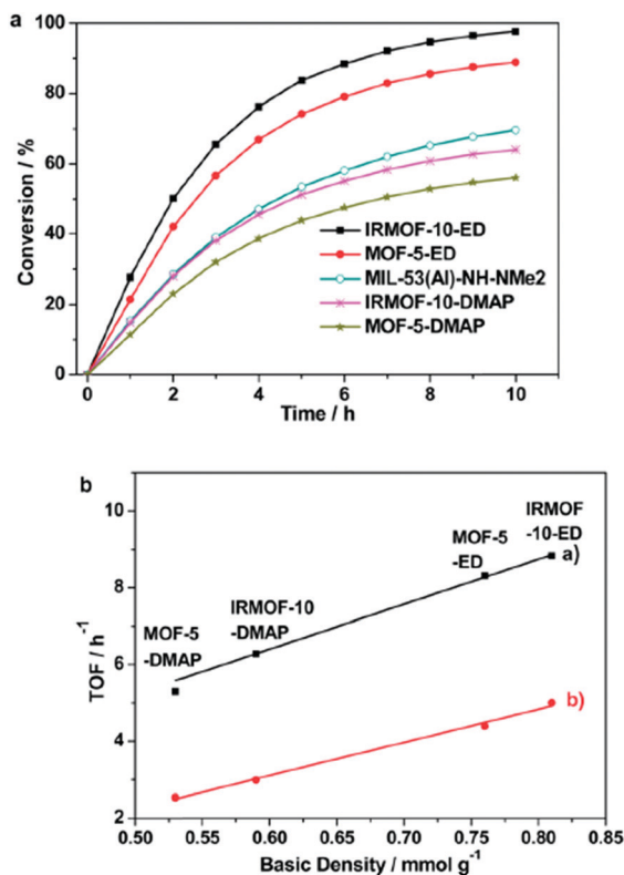
Fig. 31 (a) Comparison of the catalytic activities of amine-functionalized MOFs for the transesterification of glyceryl tributyrates with methanol (reaction conditions: glyceryl tributyrates 2.1 g; methanol 8.0 mL; catalyst 80 mg, temperature 60 °C). (b) Linear correlations between the basic site density of amine-functionalized MOFs with their catalytic activity in the transesterification of (a) glyceryl triacetate (black line) and (b) glyceryl tributyrates (red line) with methanol. Reprinted from ref. 164. Copyright 2014 with permission from the Royal Society of Chemistry.
