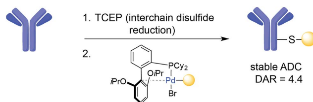
Fig. 4 Example of Cys arylation using an organometallic palladium reagent on trastuzumab.
