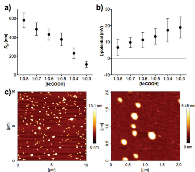
Fig. 2 (a) Hydrodynamic diameter ( D_h ) and (b) ζ-potential of P1 SH PIC nanoparticles prepared at different N : COOH ratios. (c) AFM characterisation of PIC nanoparticles prepared at a 1 : 0.3 N : COOH ratio. D = 127 \pm 42 nm, n = 48 .
