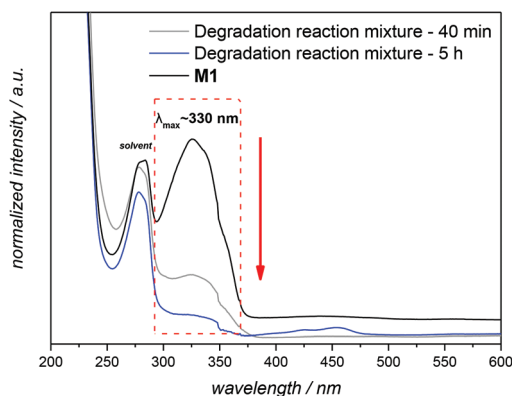
Fig. 4 UV-visible spectra illustrating the degradation of M1 in the presence of 5.5 equivalents of Na 2 S 2 O 4 in a mixture of dichloromethane: methanol: water at reflux temperature (for details see section A.8 in the ESI†). Spectra recorded in THF at 25 °C.
