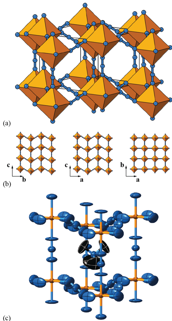
Fig. 6 Static shift distortions in [NMe 4 ]Ca[N 3 ] 3 . (a) A polyhedral/ball-and-stick representation of the crystal structure of [NMe 4 ]Ca[N 3 ] 3 , as reported in ref. 48. Ca atoms are shown in yellow and N atoms in blue. The [NMe 4 ] + cations have been omitted for clarity. Shifts are polarised along c (the vertical axis in this representation) and are related to those illustrated originally in Fig. 2(a). (b) 2D sections of the crystal structure using the same representations as in (a). These sections lie perpendicular to the a , b , and c axes (left–right) and relate the 2D shift systems enumerated in Fig. 3 with the matrix representation of the full 3D shift system active in this material. (c) A representation of the local environment of the [NMe 4 ] + cation in this material; colours are as for (a) and (b), with C atoms shown in black and H atoms omitted for clarity. Thermal ellipsoids are given at 50% probability. There is a close match in A-site cation geometry and the framework distortion effected by shift activation. The relatively large thermal ellipsoids suggest substantial dynamic disorder in this system.
