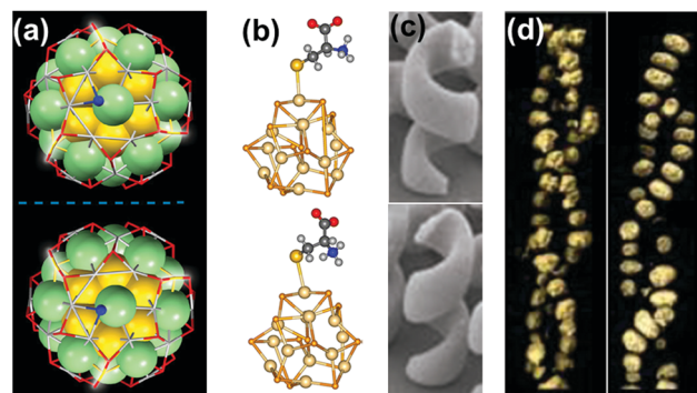
Fig. 1 Chirality in metallic, semiconductor and plasmonic nanostructures and assemblies: (a) X-ray structure of enantiomers of [\text{Ag}_{46}\text{Au}_{24}(\text{SR})_{32}](\text{BPh}_4)_2 NCs. Reproduced with permission from ref. 58. Copyright 2015 American Association for the Advancement of Science. (b) Optimized geometries of L- and D-cysteine capped semiconductor CdSe nanocrystals. Reproduced with permission from ref. 74. Copyright 2013 American Chemical Society. (c) TEM images of left- and right-handed gold nanohelices. Reproduced with permission from ref. 89. Copyright 2009 American Association for the Advancement of Science. (d) TEM tomography images of left- and right-handed gold NP double helices formed on a peptide template. Reproduced with permission from ref. 132. Copyright 2013 American Chemical Society.
