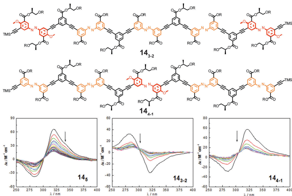
Fig. 18 Photoswitchable heterogeneous oligoazobenzene tetradecamers 14 3-2 and 14 4-1 ( R = -(CH_2CH_2O)_3CH_3 ) and the corresponding CD spectra ( 14 5 shown for comparison) during the course of irradiation at \lambda_{irr} = 358 nm in CH_3CN at 25 °C. 108
