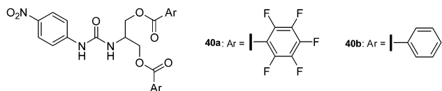
Fig. 20 Molecular structure of the urea-based receptors as used by Taylor for studying anion- \pi and halogen bonding in solution. 43
