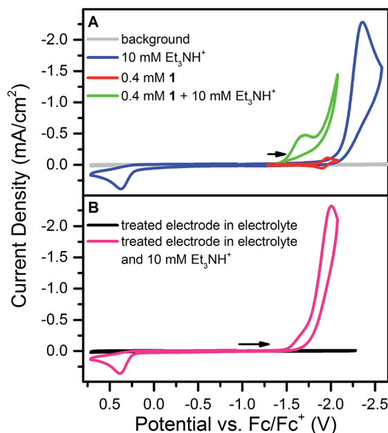
Fig. 2 (A) Cyclic voltammograms of [\text{Et}_3\text{NH}][\text{BF}_4] , 1 , and 1 plus [\text{Et}_3\text{NH}][\text{BF}_4] at 100 \text{ mV s}^{-1} in 0.25 \text{ M } [\text{Bu}_4\text{N}][\text{PF}_6] . (B) Cyclic voltammograms using an electrode treated at -1.78 \text{ V} for 60 \text{ s} with 0.4 \text{ mM } \mathbf{1} and 10 \text{ mM } [\text{Et}_3\text{NH}][\text{BF}_4] , rinsed, and then scanned in a solution of 0.25 \text{ M } [\text{Bu}_4\text{N}][\text{PF}_6] (black line) and in a solution of 10 \text{ mM } [\text{Et}_3\text{NH}][\text{BF}_4] + 0.25 \text{ M } [\text{Bu}_4\text{N}][\text{PF}_6] (pink) at 100 \text{ mV s}^{-1}
