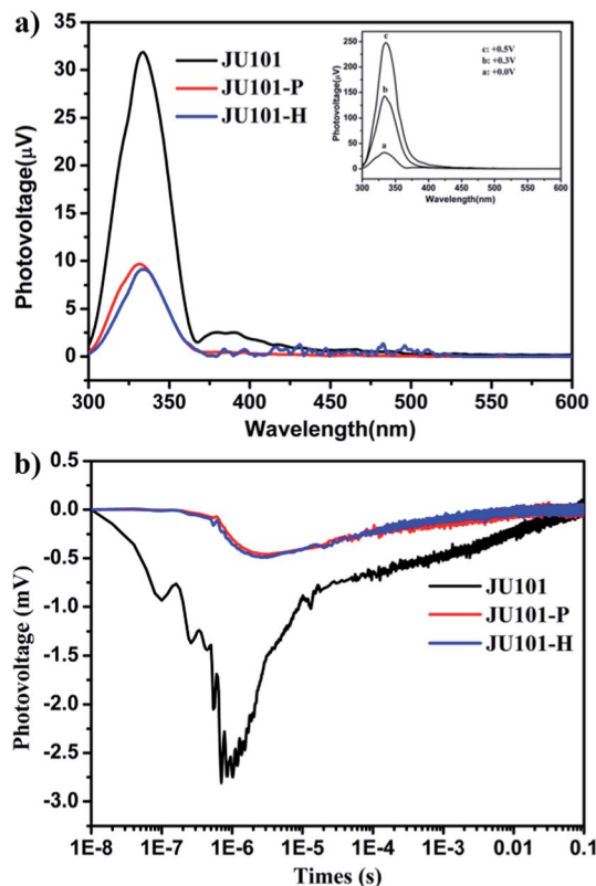
Fig. 4 (a) SPV spectra of JU101, photo irradiated sample JU101-P and heated sample JU101-H in the absence of an external electric field. Inset: FISPS of JU101 under different positive electric-fields. (b) TPV spectra of JU101, JU101-P, and JU101-H.
