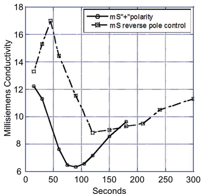
Fig. 31 Electrodesorption process for the capacitor based on an ionic group derivatized nanoporous carbon electrode charged in the positive polarity and scientific control capacitor (Reproduced with permission from ref. 132.)
