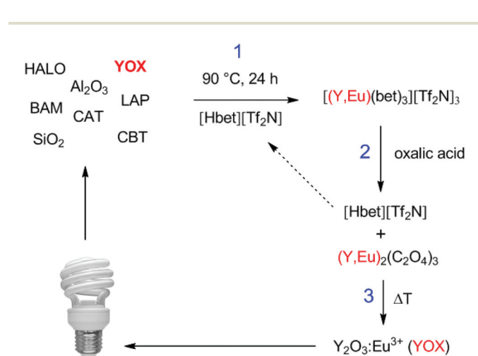
Fig. 13 Overview of the proposed recycling process for lamp phosphor waste, based on the selective dissolution and revalorization of YOX with the protonated functionalized ionic liquid [Hbet][Tf_2N] . Step 1: selective dissolution of YOX, step 2: stripping with pure oxalic acid (regenerates the ionic liquid), step 3: direct resynthesis of YOX.
