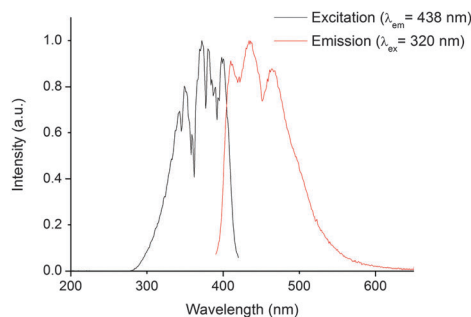
Fig. 2 Steady state excitation spectrum (black trace, recorded at the emission maxima of 438 nm), and emission spectrum (red trace, recorded following 320 nm excitation), of 1 in CH 2 Cl 2 at 295 K.
