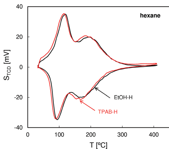
Fig. 4 QE-TPDA profiles of hexane measured for the studied ZSM-5 zeolites at 10\text{ °C min}^{-1} .
