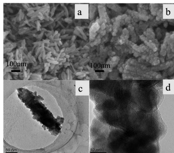
Fig. 5 SEM images of the as-prepared TiO 2 nanorod film before (a) and after (b) coating with CdS nanoparticles at high magnification; TEM image of a single CdS/TiO 2 core/shell nanorod (c) and high-resolution TEM image of a single CdS/TiO 2 core/shell nanorod (d) (reprinted with permission from ref. 45, copyright 2007 Elsevier).
